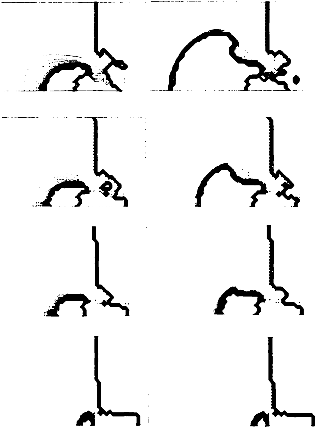
Figure 11b. Contours of Constant Mass Fraction Following Impact of 3.30 mm (0.13 in.)-diam Cylinder at 2093 m/s (6967 ft/s), at Top and 2178 m/s (7146 ft/s), at Bottom at 0.42, 1.26, 1.68, and 2.11 \mu\text{s}
