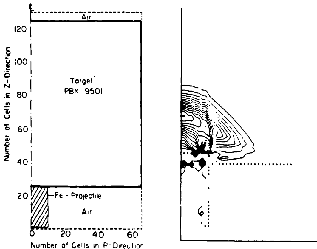
Figure 3. Typical Computer Model for an Impinging Cylindrical Projectile
