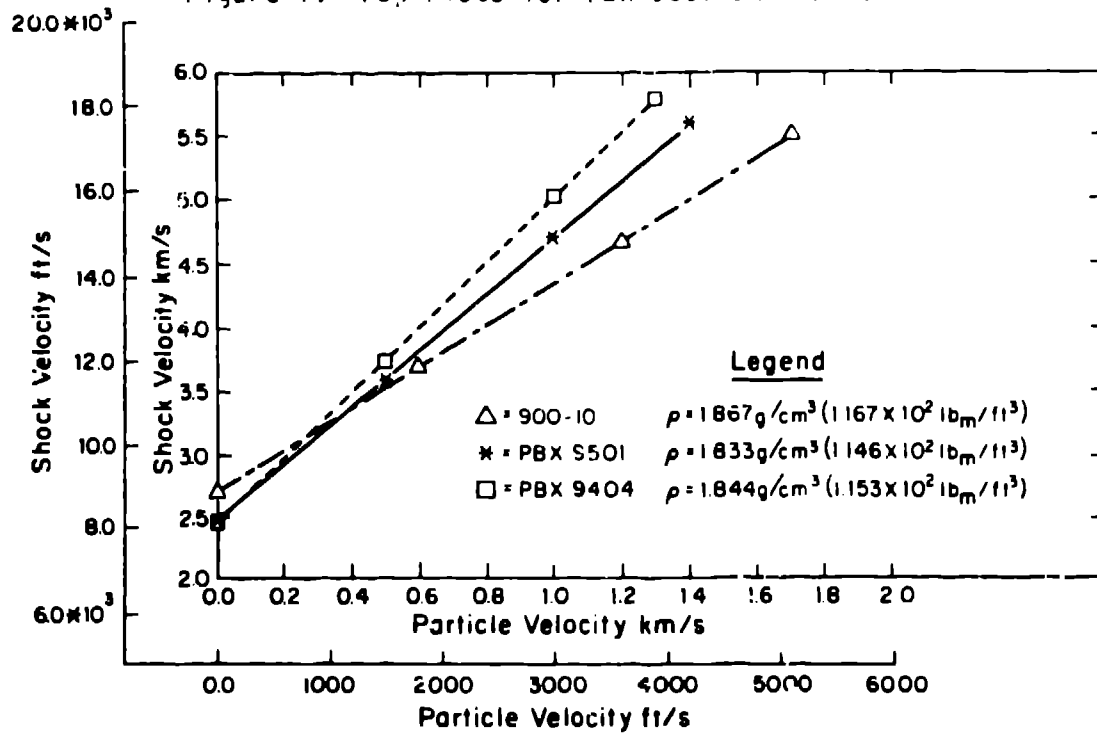
Figure 2. Shock-Particle Velocity Relation for 900-10, PBX 9501, and PBX 9404
